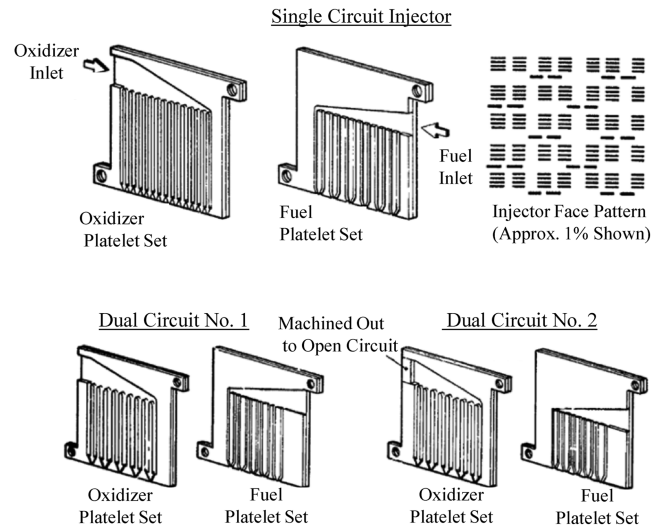
Fig. 14 HIPERTHIN platelet dual-manifold injector design [66].
