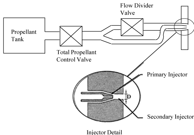
Fig. 9 Dual-manifold injection flow system schematic [45–47].
