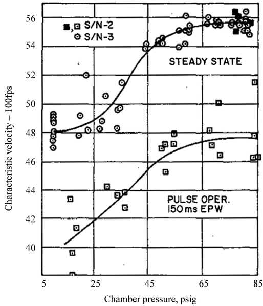
a) Comparison of steady and pulsing performance
