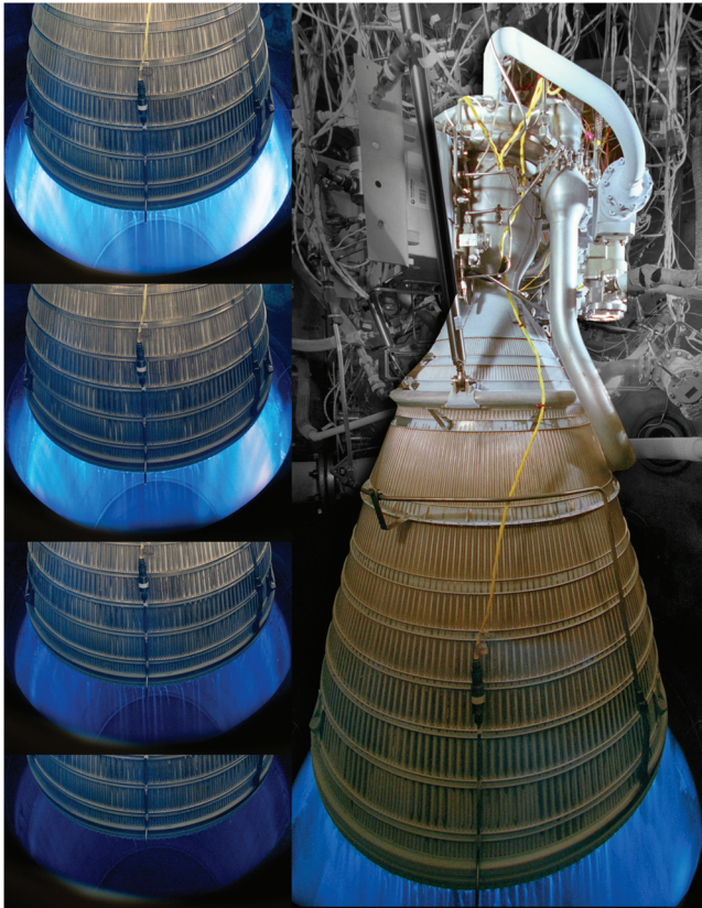
Fig. 6 CECE shown at multiple power levels [41].
