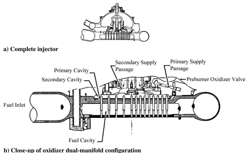
Fig. 12 XLR-129 dual-manifold preburner configuration [54–65].
