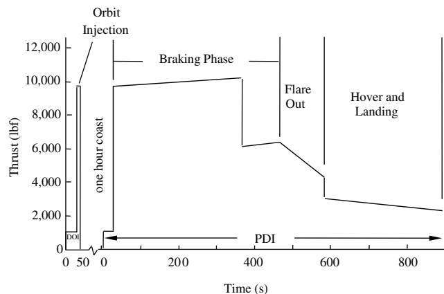
Fig. 25 LMDE nominal duty cycle [19,78,100-103].
