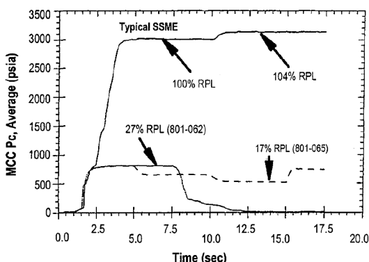
Fig. 5 SSME low power level chamber pressure [37,38].
