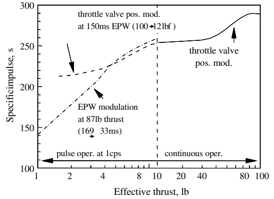
Fig. 20 Dual-mode throttling performance [91].
