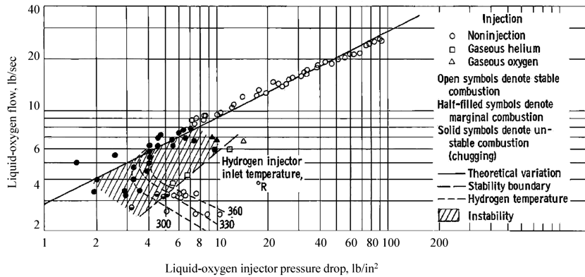
Fig. 4 Hydraulic characteristics with throttling of a liquid oxygen shear coaxial injector [29].
