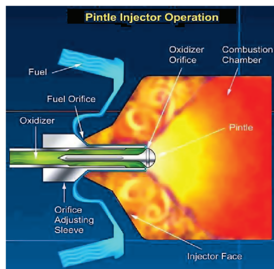
Fig. 29 Pintle injector operation illustration [113–115].
