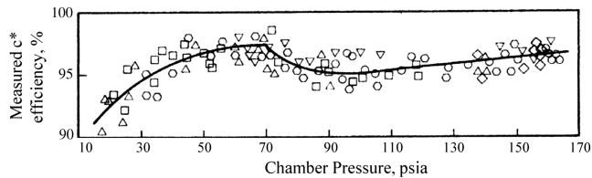
Fig. 11 Dual-manifold throttling performance with series valve configuration [50]; propellants: FLOX/MMH; mixture ratio: 1.79:2.36; chamber length (injector throat): 10.32 in.; test number: 2 ○, 3 □, 4 ◇, 5 △, 6 ○, 7 ▽.
