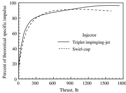
Fig. 24 Theoretical specific impulse for triplet impinging-jet variable area injector [99].
