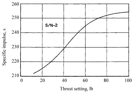
c) Pulsing performance at 150 msec pulse-width
