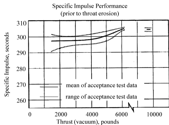
Fig. 27 LMDE engine specific impulse before throat erosion [100].
