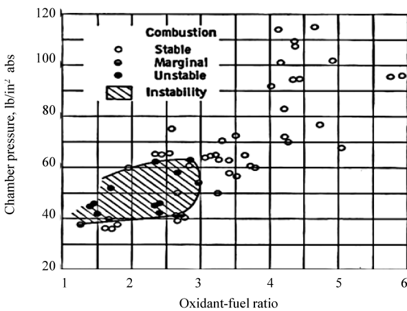
c) High-pressure-drop injector
