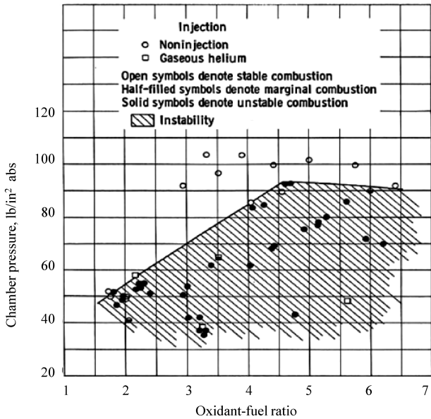
a) Low-pressure-drop injector
