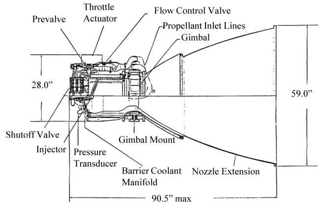
Fig. 26 LMDE engine layout [100,101].
