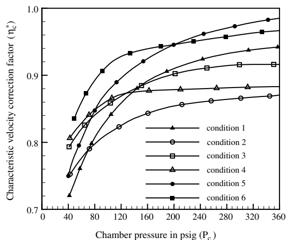
Fig. 1 Characteristic velocity efficiency from Project Thumper [27].
