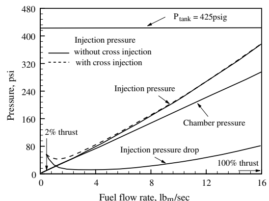
Fig. 15 System pressures versus fuel flow rate with a constant secondary mixture ratio [75].
