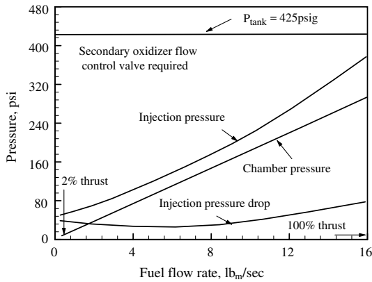
Fig. 16 System pressures versus fuel flow rate with a constant secondary oxidizer pressure [75].
