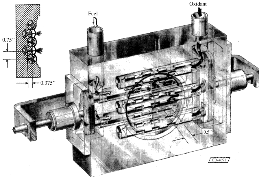
Fig. 22 Triplet impinging-jet variable area injector [99].
