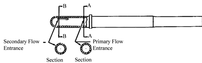
Fig. 13 XLR-129 dual-inlet swirl coax oxidizer element [54–65].
