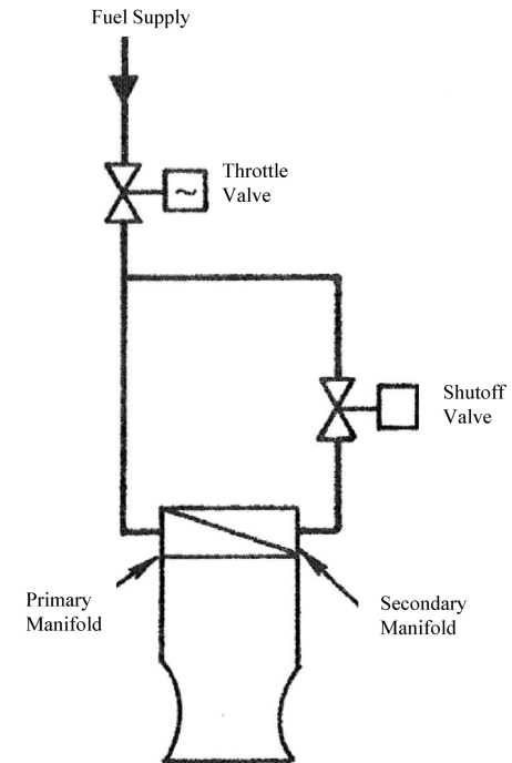
a) Parallel scheme
