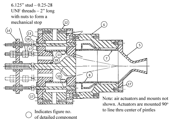
Fig. 28 Gaseous propellant variable area injector engine schematic [108].
